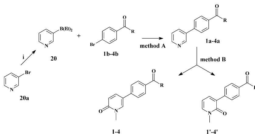
Scheme 1. Synthesis of 5-phenyl and 3-phenyl substituted 1-methyl-2-pyridones 1–4 and 1'–4' .
