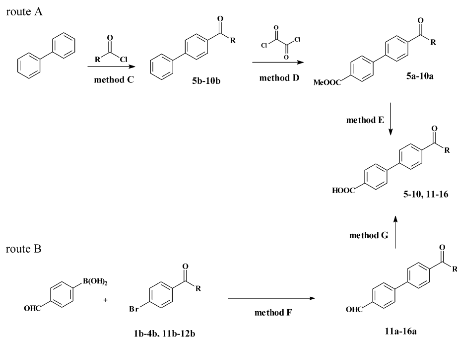
Scheme 2. Synthesis of 4'-substituted biphenyl-4-carboxylic acids 5–16 .
